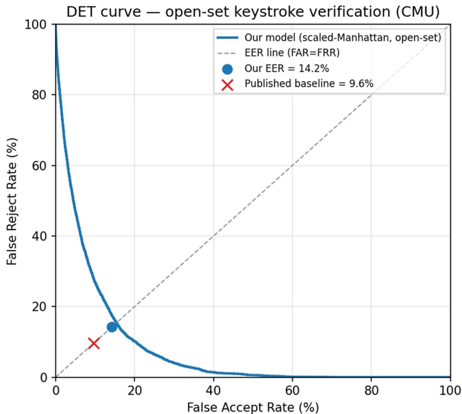
Figure B.1: the error trade-off (DET curve).
